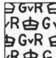
Block Cypher
